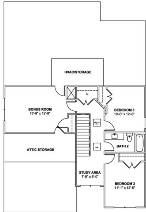
UPPER LEVEL
