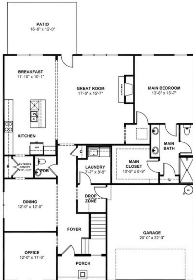
MAIN LEVEL
