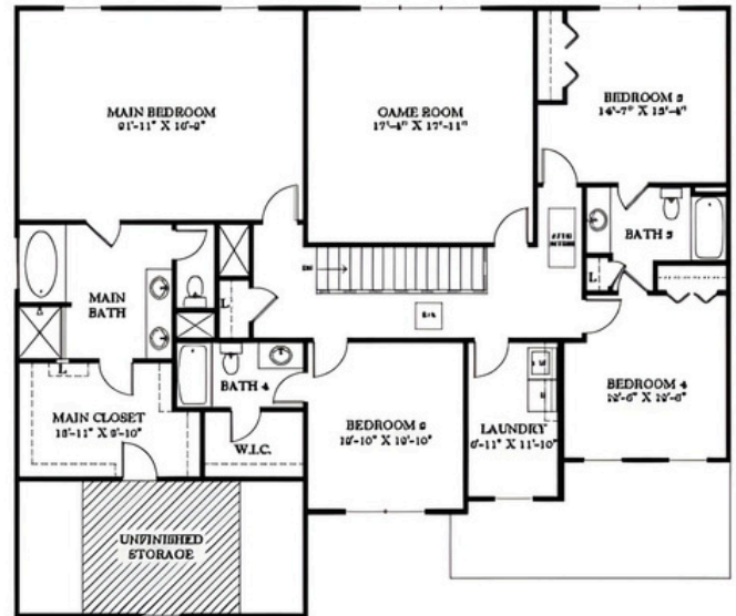
UPPER LEVEL
