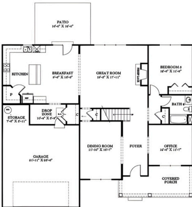
MAIN LEVEL
